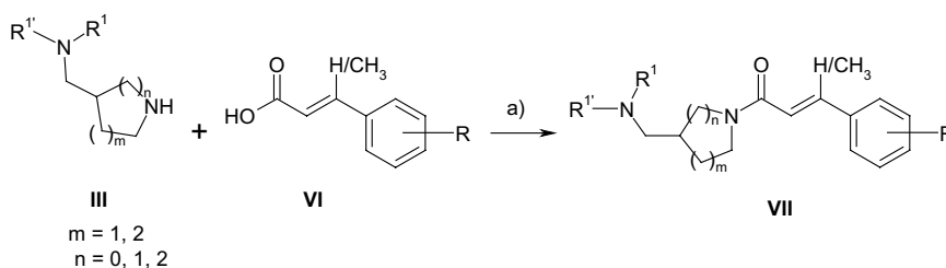
Scheme 4. (a) EDAC, DHOBT, \text{Et}_3\text{N} .
