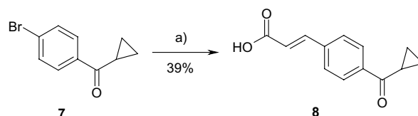
Scheme 3. (a) (i) \text{Pd}(\text{PPh}_3)_4 , \text{CH}_2=\text{CHCOOEt} , \text{NEt}_3 ; (ii) \text{LiOH} , dioxane/water.
